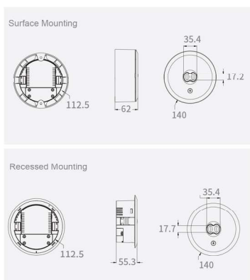
sizes
