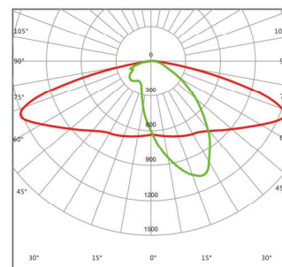
photometric diagrams
